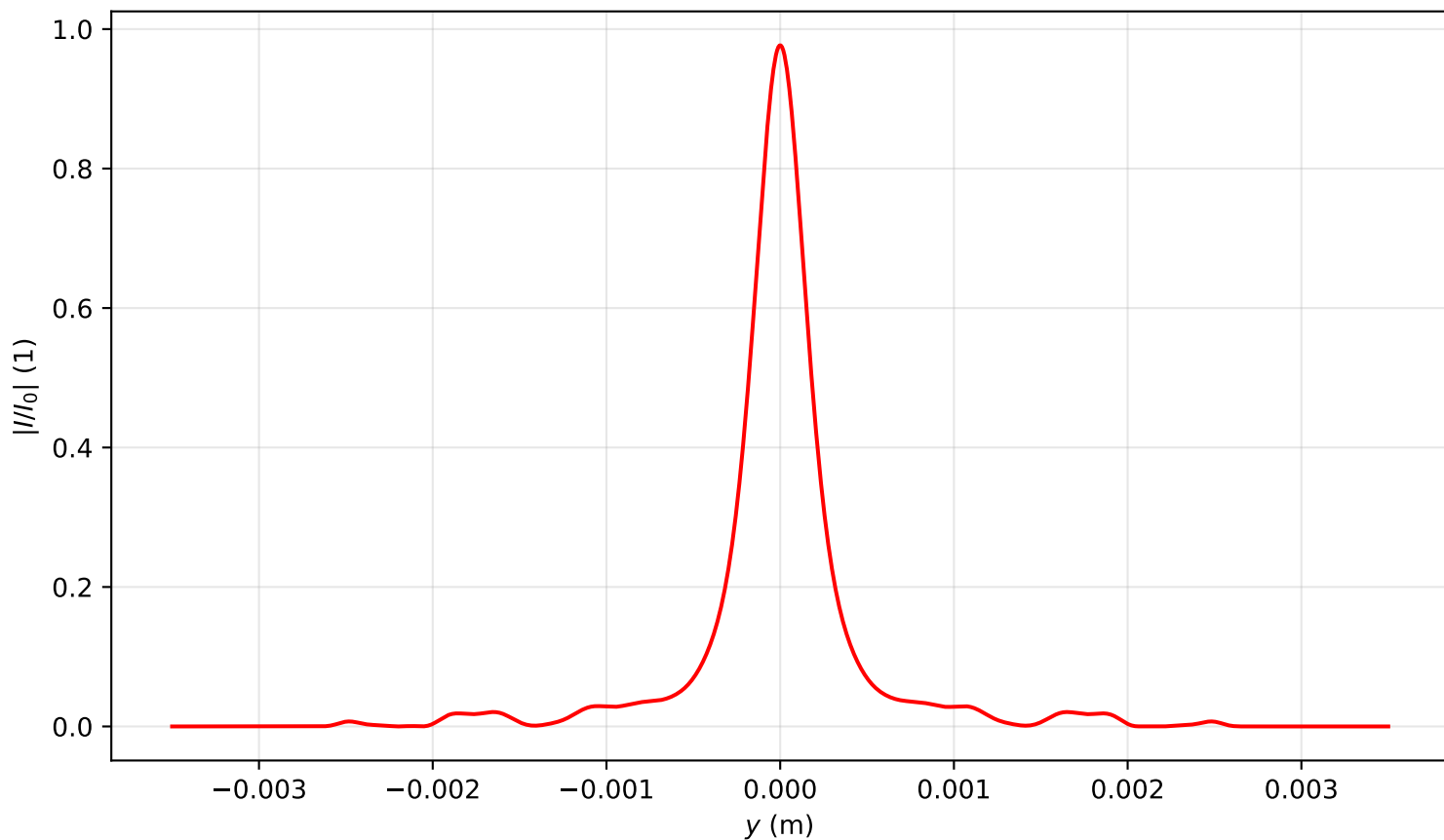
Intensity profile I(x=0, y, z=3.105)/I_0 , P_{in}=4.0P_{cr} , artificial time
